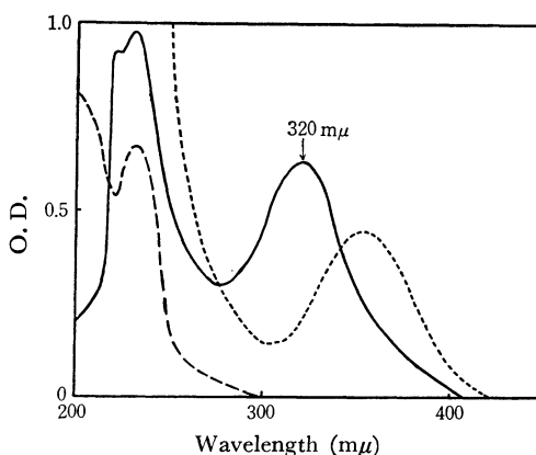
Fig. 1. The absorption spectra of N^\alpha, N^\omega, N^{\omega'} -tricarbobenzyloxy-L-arginine- p -nitroanilide, N^\alpha, N^\omega, N^{\omega'} -tricarbobenzyloxy-L-arginine and p -nitroaniline in dioxane.
